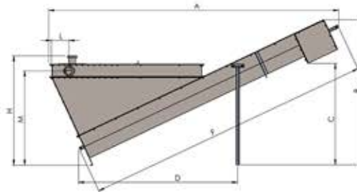
Grit Separator-technical specification, mm
